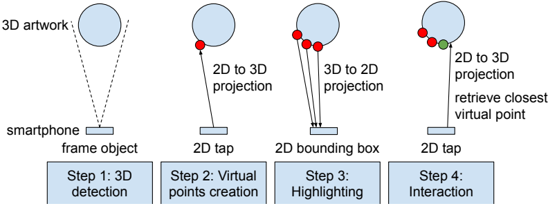
(a) Highlighting and touchscreen interaction
