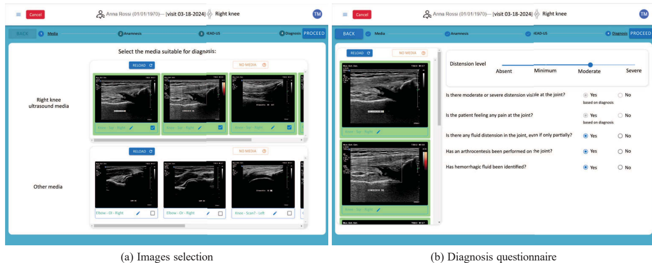
Fig. 4: CADET interface
